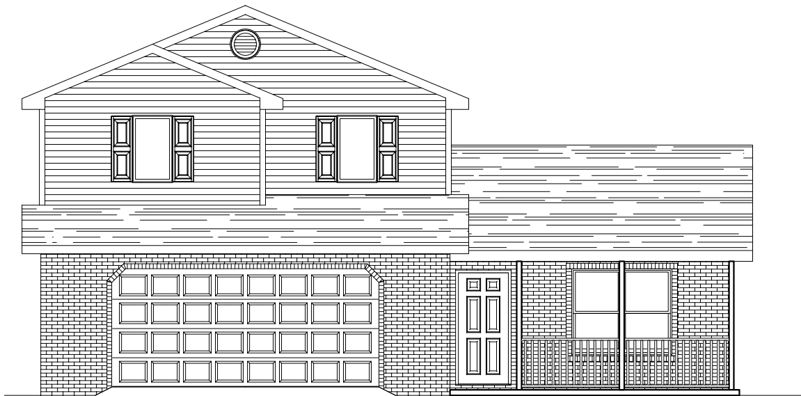
ELEVATION "A"
