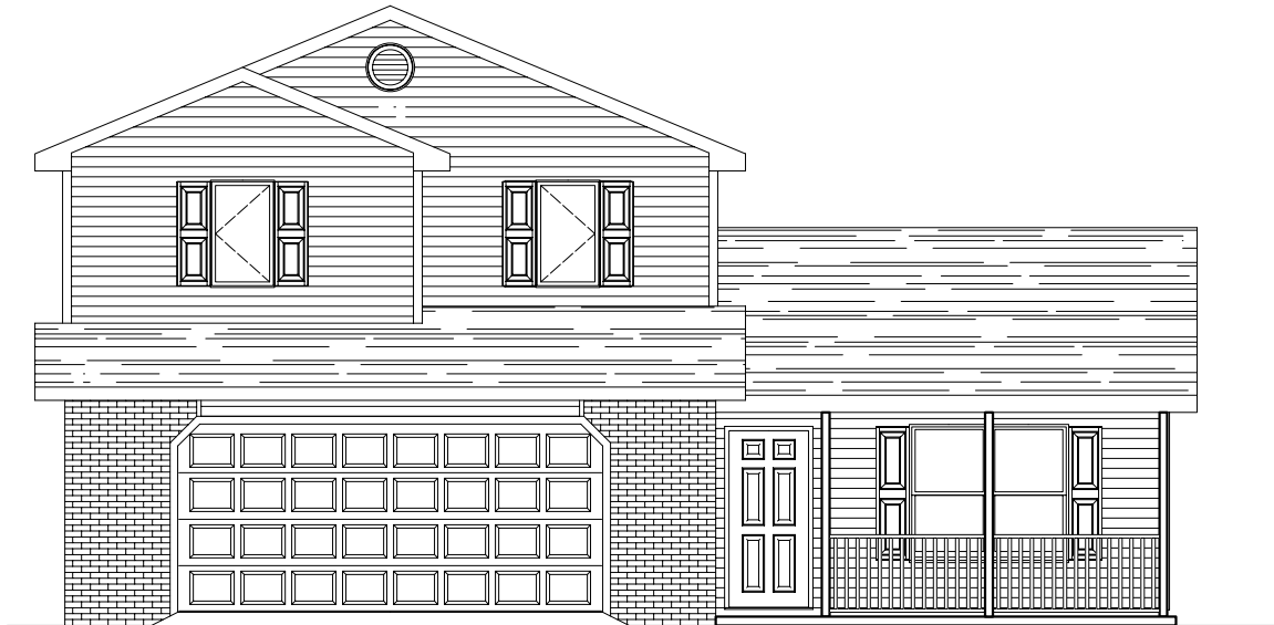
ELEVATION "A"
