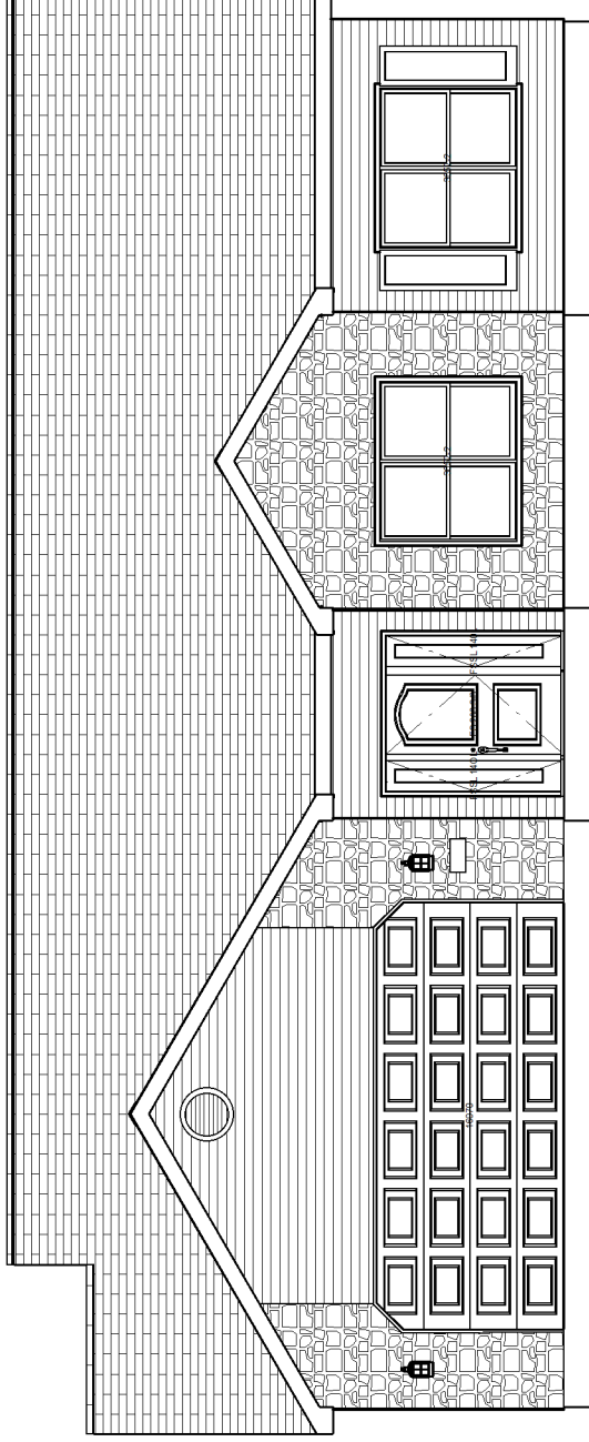
Elevation A SHOWN WITH OPTIONAL SIDELIGHTS AND STONE
