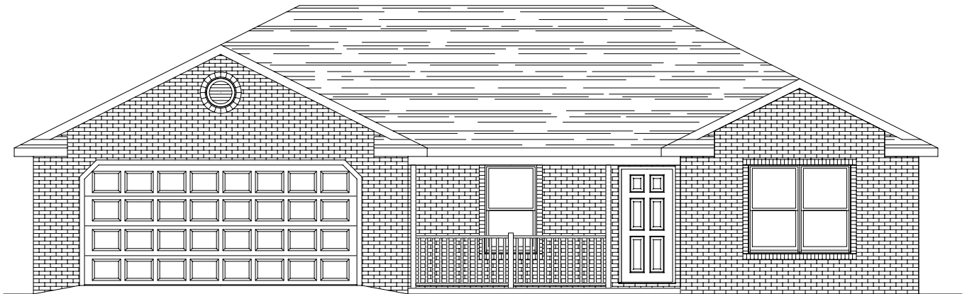
ELEVATION "D"
